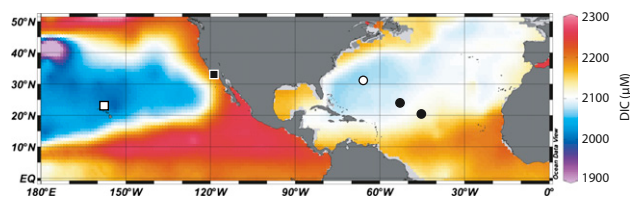
Fig. 1. Experiment locations overlaid on dissolved inorganic carbon (DIC) concentrations at 200 m depth from Goyet et al. (52). The location of the HOT experiments is denoted by the white square, the SPOT experiment is denoted by a black square, BATS is denoted by a white circle, and the locations of the two Sargasso Sea experiments are denoted by black circles.
