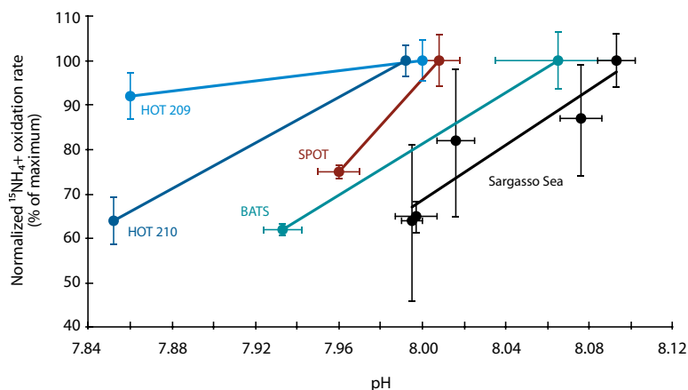
Fig. 3. Correspondence between ammonia oxidation rates and \text{pH}_{\text{total}} for all experiments. Ammonia oxidation rates were renormalized to the maximum rate measured in the experiment. For the Sargasso Sea regression line, y = 310x - 2,410 , r^2 = 0.87 , and P < 0.05 . Calculated \text{pH}_{\text{total}} values are shown for HOT 209, and error bars denote 1 SD among triplicate treatments, except in the case of rate measurements in the Sargasso Sea, where error bars denote the SE of triplicate measurements.
