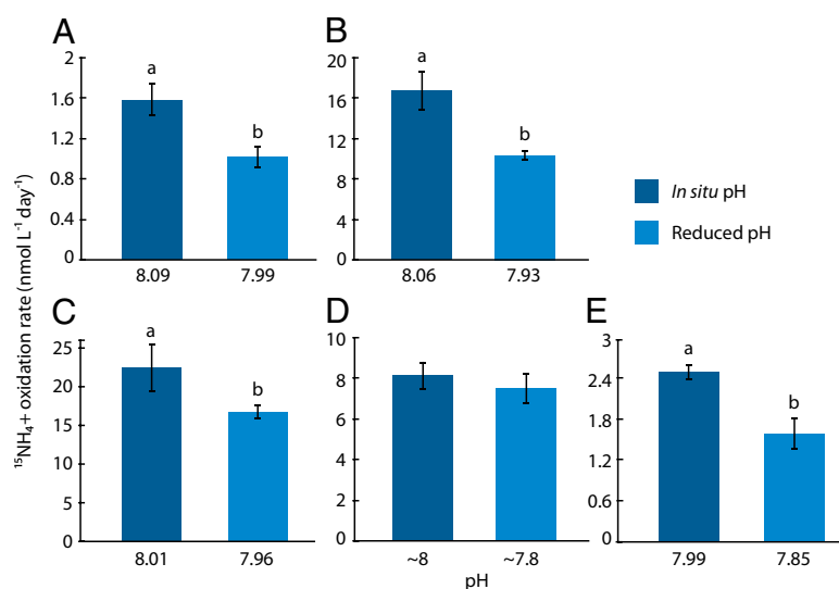
Fig. 2. Reductions in ammonia oxidation rates in ocean acidification experiments in (A) the Sargasso Sea, at (B) BATS, at (C) SPOT, at (D) HOT 209, and at (E) HOT 210. \text{pH}_{\text{total}} values are noted along the horizontal axis (calculated \text{pH}_{\text{total}} values are shown for the HOT 209 experiment). Statistically significant differences among means ( P < 0.05 ) were determined via one-way ANOVA, and error bars denote 1 SD of triplicate treatments. Ammonia oxidation rates at SPOT were calculated from the linear accumulation of ^{15}\text{N} label in the oxidized pool over the course of the experiment; all other values represent end-point measurements.
