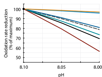
Fig. 4. Renormalized acidification-driven decreases in ammonia oxidation rates. Rate reductions are expressed as a percentage decrease in rates in acidified seawater compared with controls and are normalized to a 0.1 unit decrease in pH from 8.1 to 8. Previously reported data for > 0.5 pH changes in Huesemann et al. (8) are included for comparison and denoted by the orange line; other colors are for experiments that are identical to those in Fig. 3. The mean reduction is denoted by the dashed gray line.
